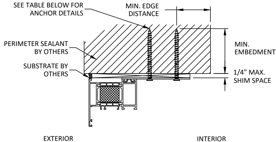
A 6 VERTICAL SECTION THROUGH STRAP INSTALLATION
